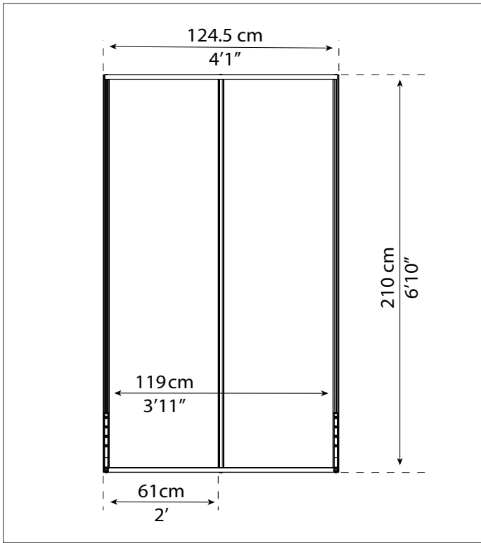
Dividers Measurements
